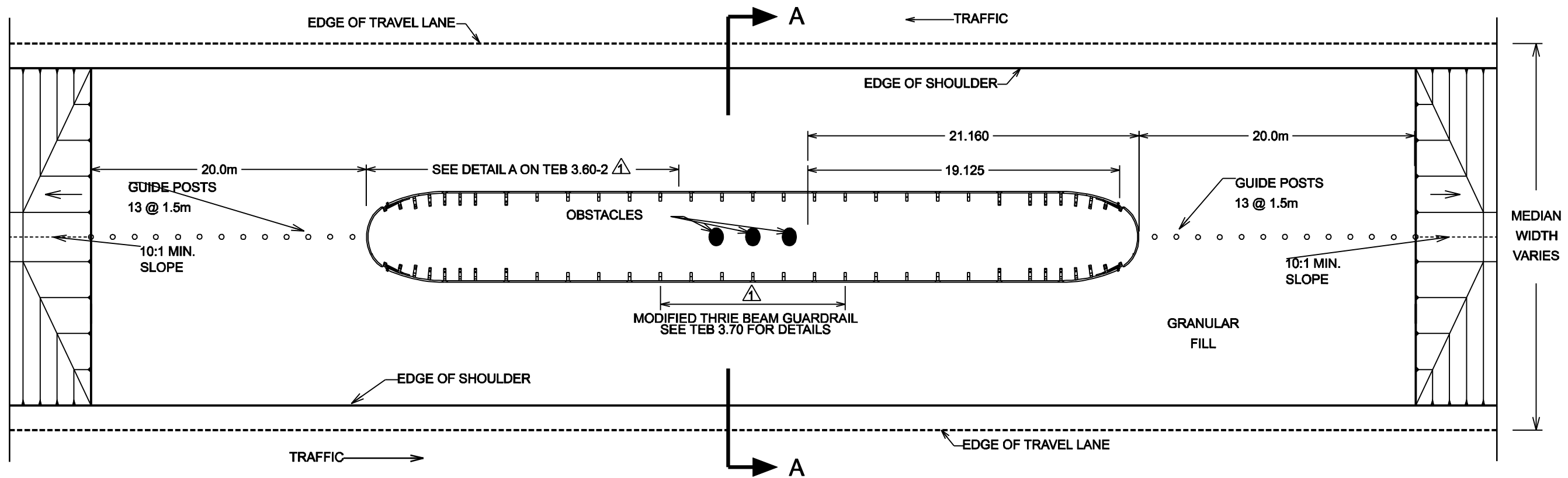
PIER AT C OF MEDIAN PLAN VIEW
