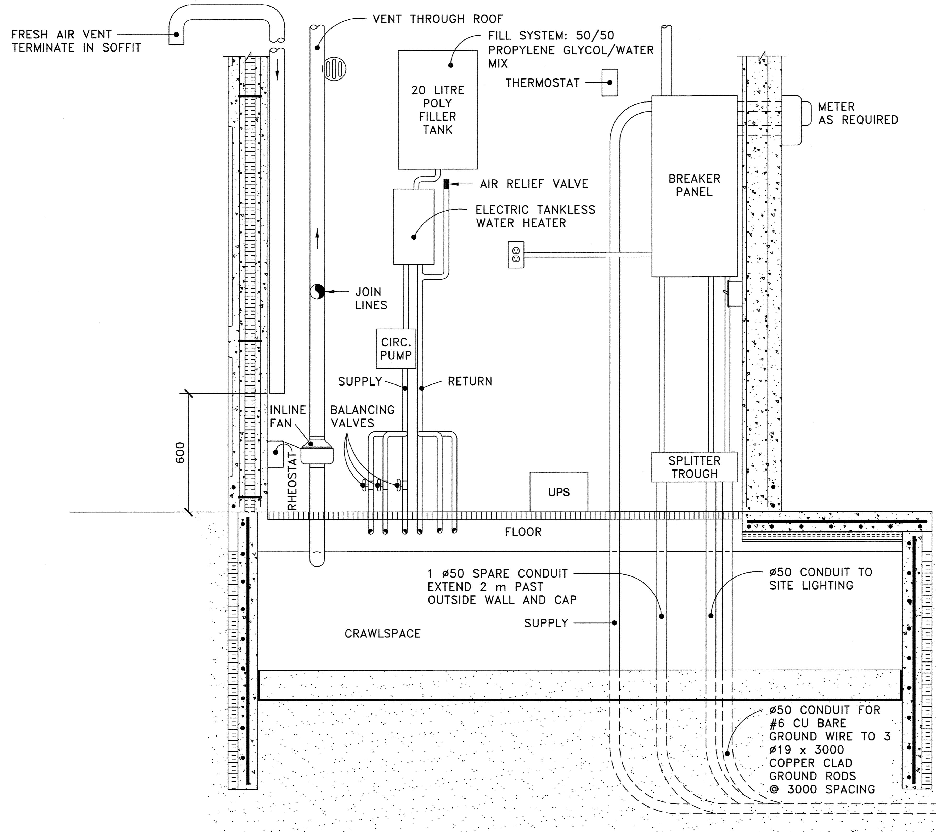
1 SECTION THROUGH MECHANICAL ROOM OF ELECTRICAL POWER TOILET CB6-4.6M15 N.T.S.
