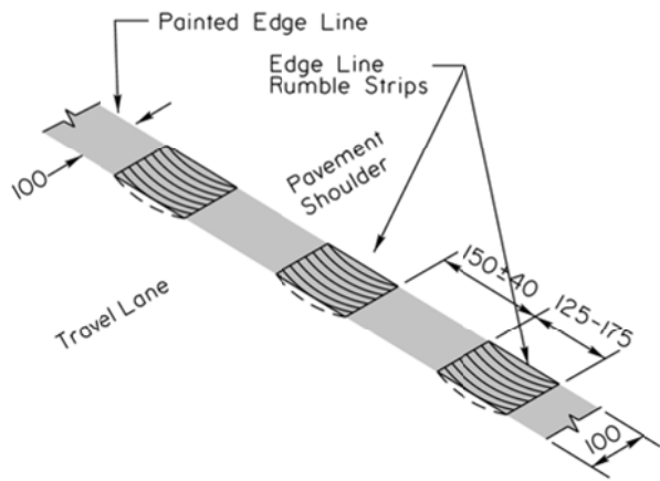
TYPICAL GAP EDGE LINE RUMBLE STRIP INSTALLATION
