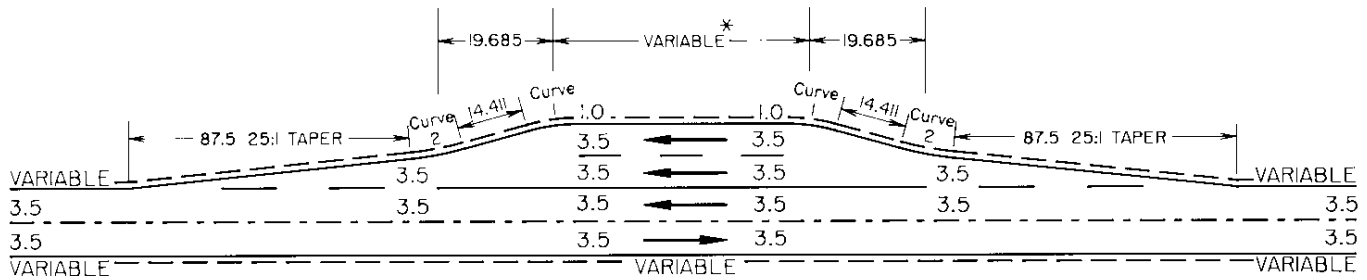
TYPICAL STANDARD PULL-OFF
