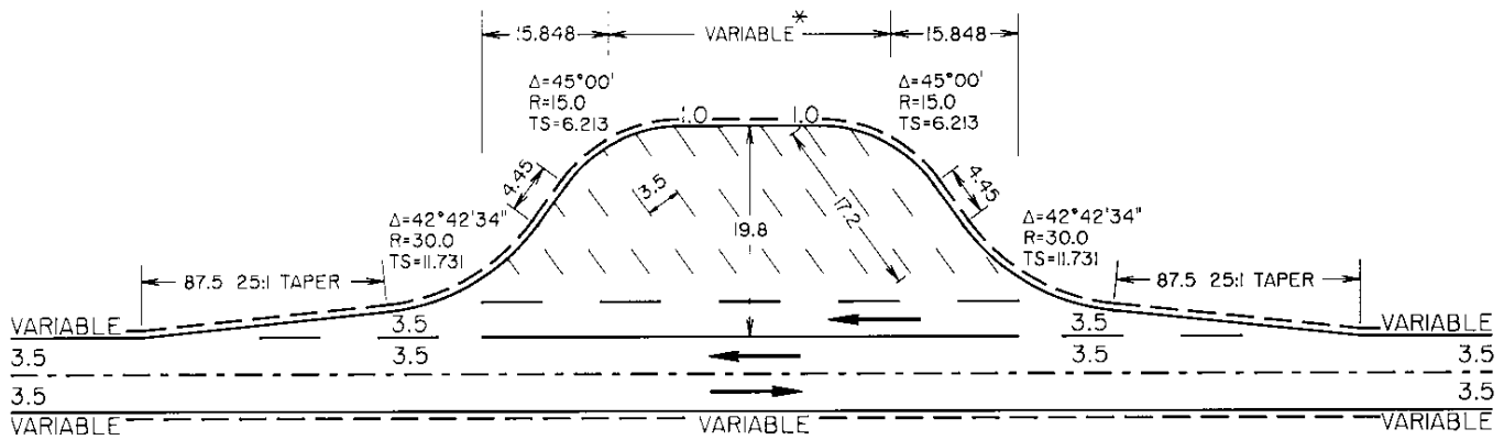
TYPICAL DEEP PULL-OFF
