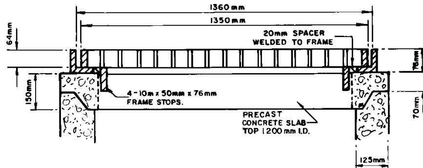
DETAIL OF FRAME AND COVER
