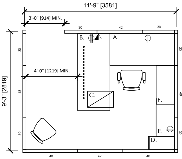
4 DIRECTOR (AND EQUIVALENT) WORKSPACE 10.1 m 2
